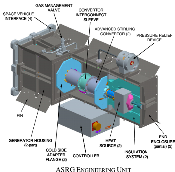
ASRG ENGINEERING UNIT
