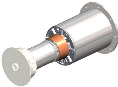
ADVANCED STIRLING CONVERTOR
