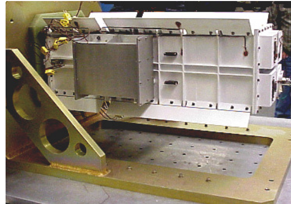
ASRG EU ON THERMAL VACUUM FIXTURE
